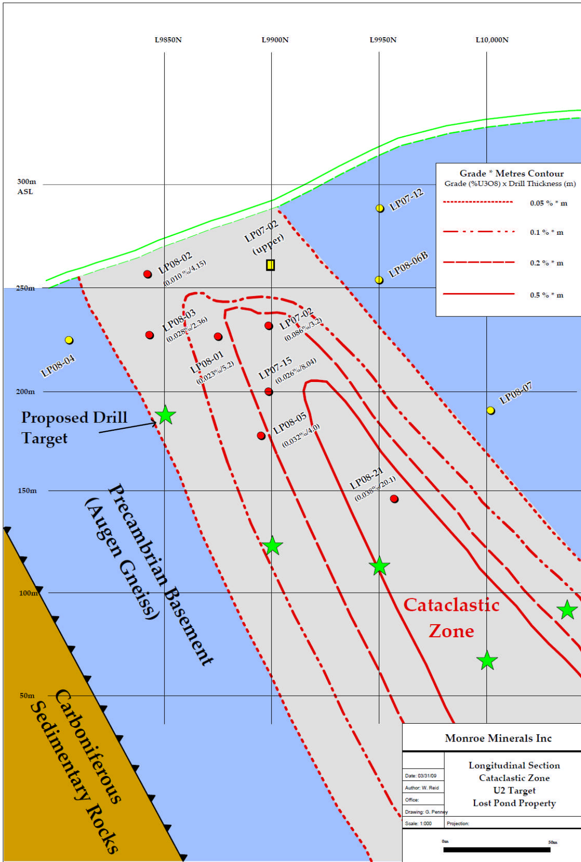
Management's interpretation of the U2 Cataclastic Zone longitudinal section.
